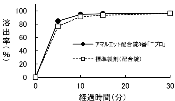
図2-5 試験液:pH 5.0 (100 rpm)
