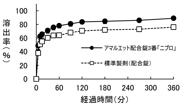
図2-3 試験液:pH 6.8 (50 rpm)
